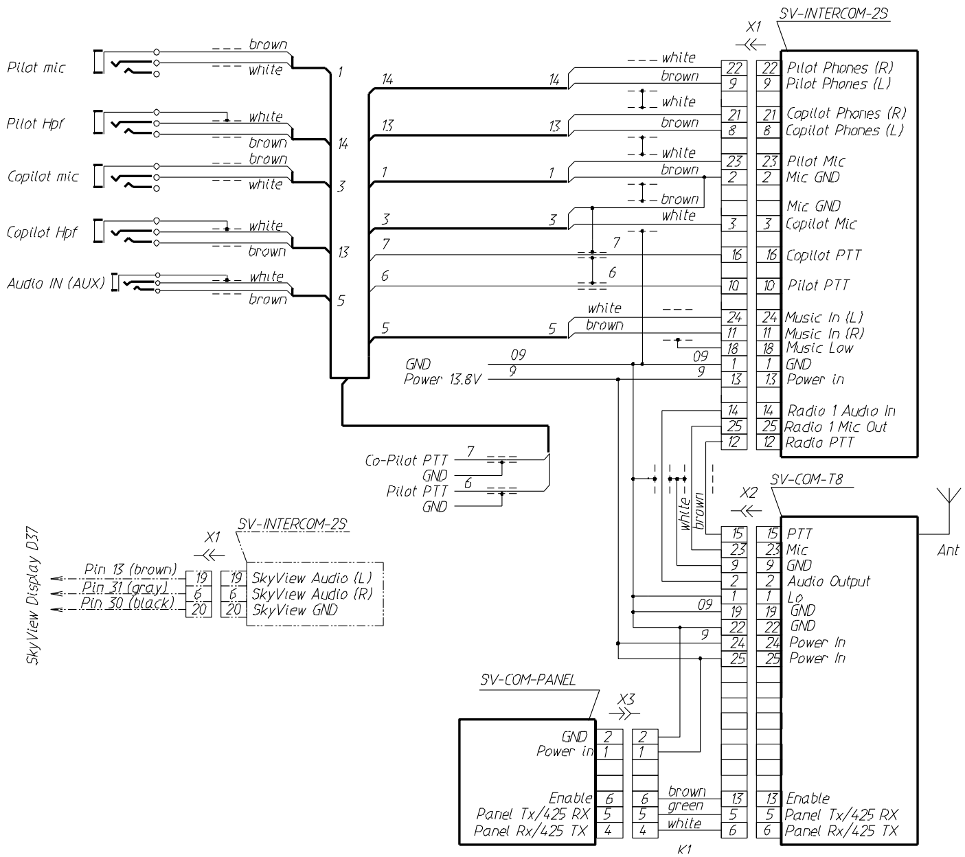
Fig. 19 Wiring diagram for Dynon SkyView T8 radio
