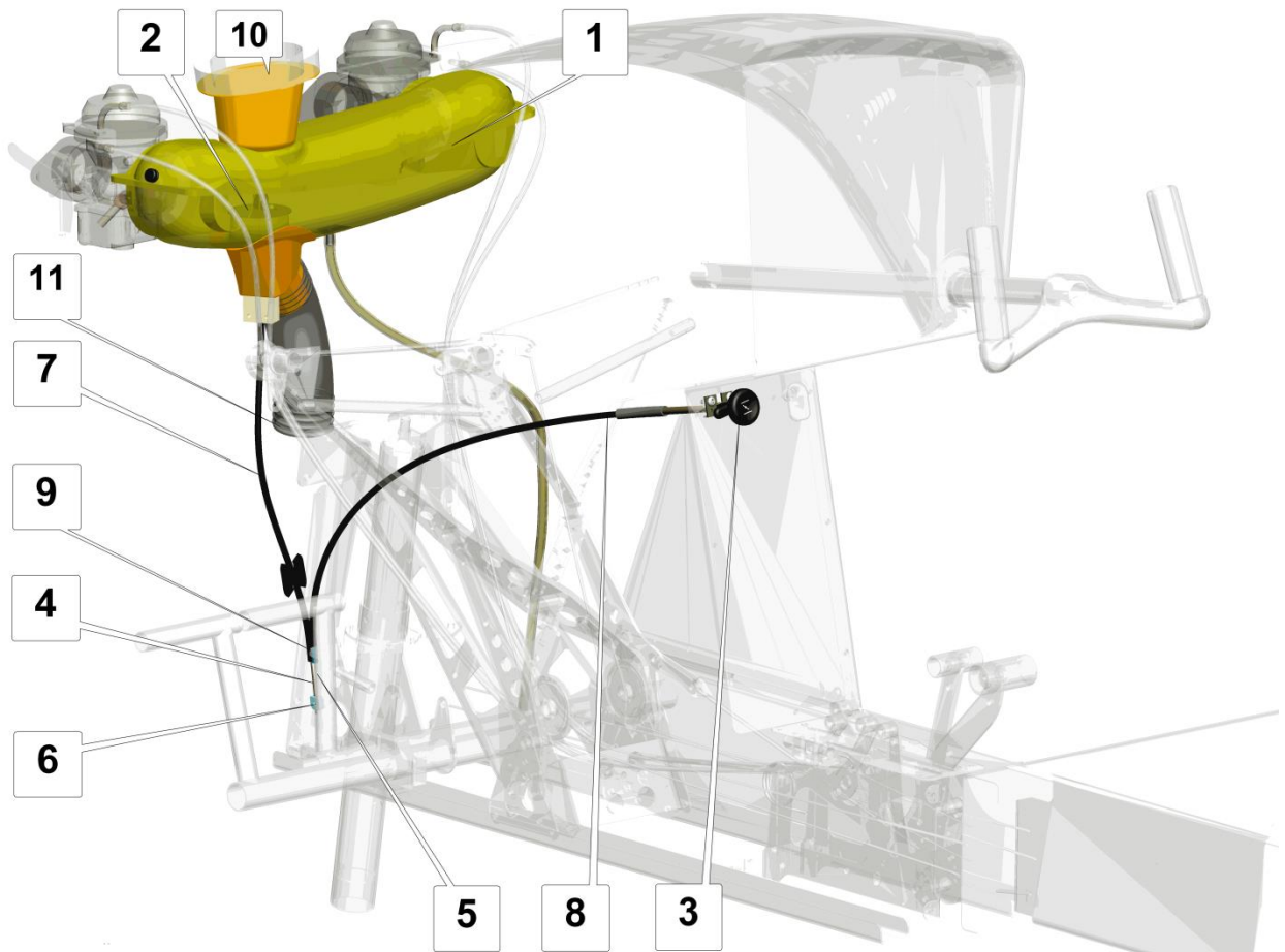
Fig. 11 Carburettor heating control
