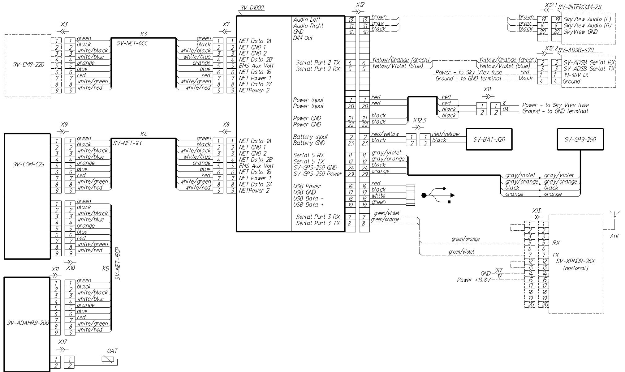
Fig. 17. Wiring diagram for installation of SkyView system (page 2)
