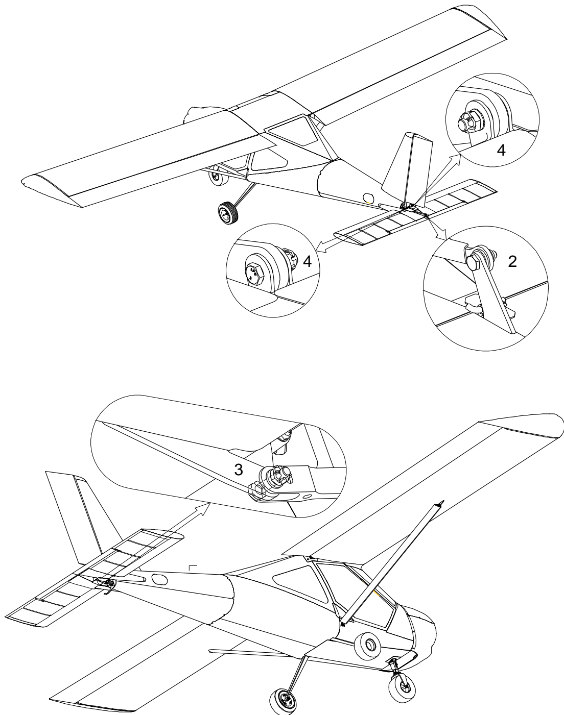
Fig. 23 Removal of the AFHT
