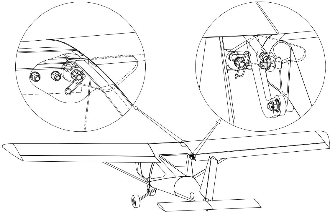
Fig. 21 Wing removal – wing-to-fuselage attachment points
