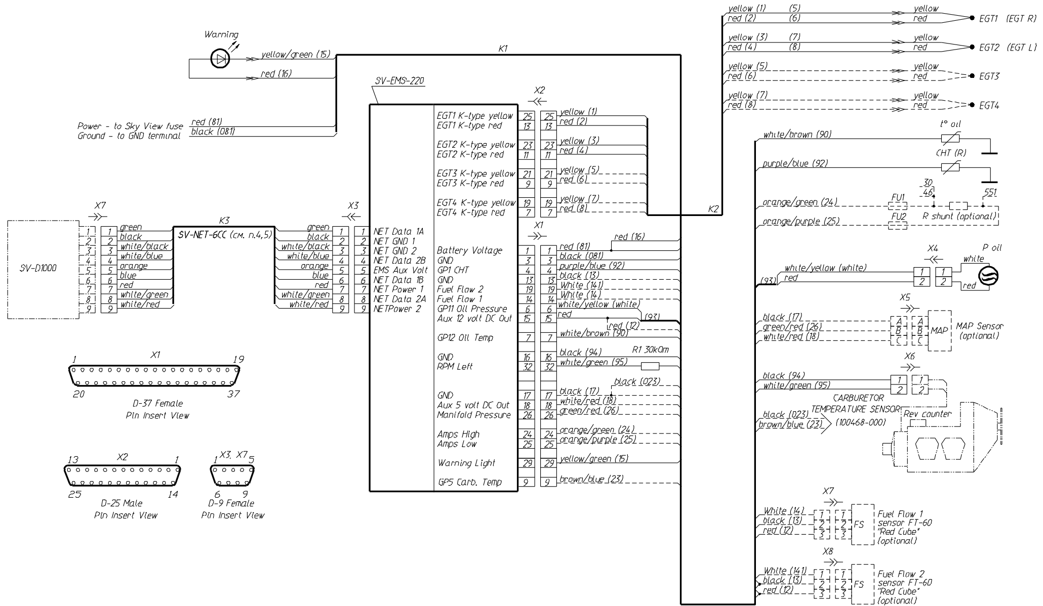
Fig. 16. Wiring diagram for installation of SkyView system (page 1)
