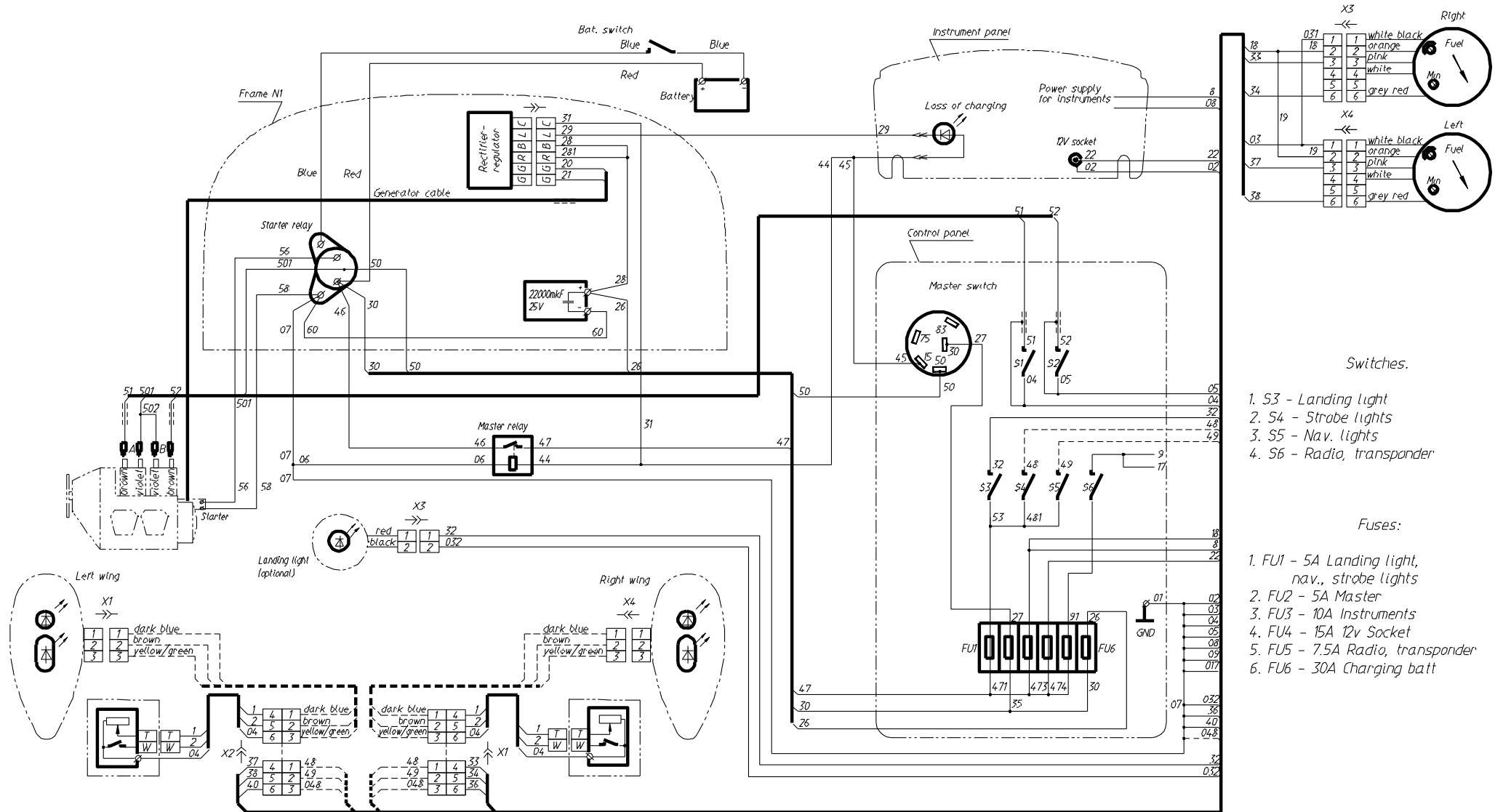
Fig. 15 Wiring diagram of A-32 electrical system (main)
