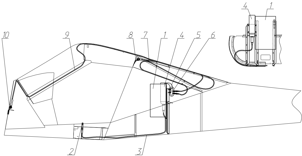
Fig. 20 Recovery system
