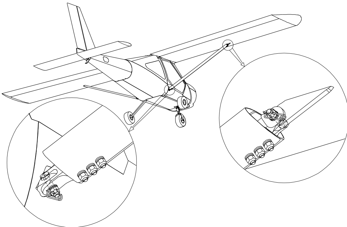
Fig. 22 Wing removal – wing strut attachment points
