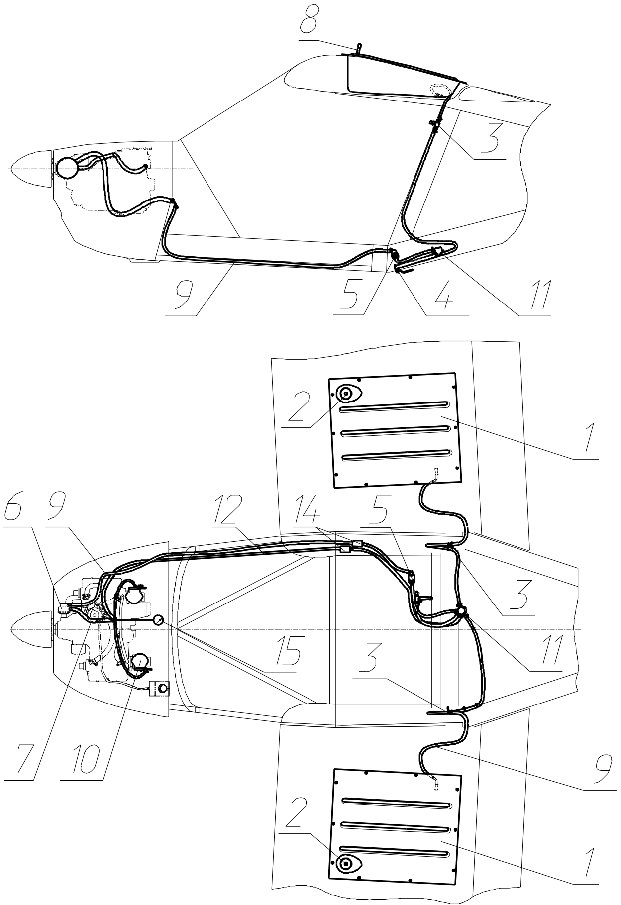
Fig. 3. Fuel system schematic
